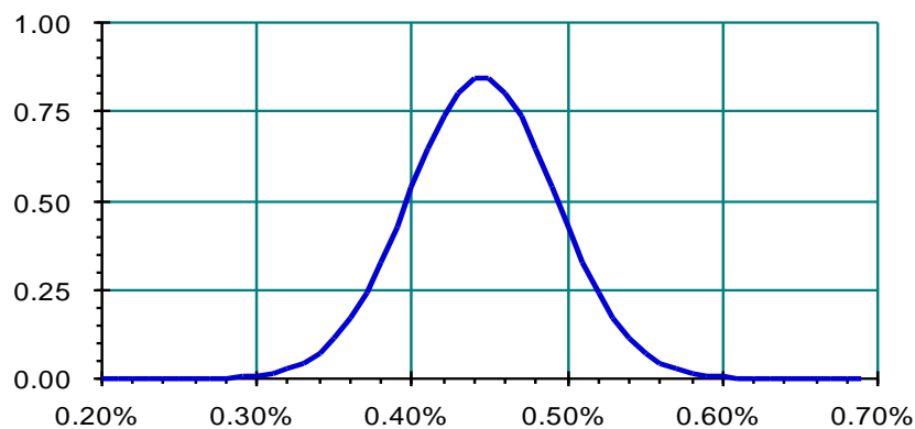
Figure VIII. 2 Gaussian distribution
